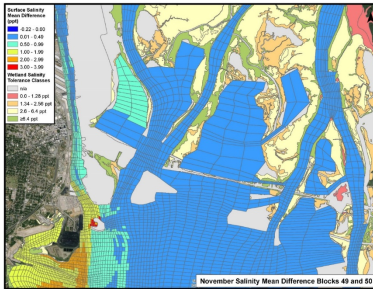
Figure 3-48. Estimated increase in salinity during the fall period (November data shown for example). Note that in areas containing wetlands estimated salinity increases are limited to 0.0, <0.5, or <1.0 ppt. In areas where increases may occur, wetland communities are adapted to predicted conditions. Higher increases in salinity (e.g., >2 ppt) may occur adjacent to the navigation channel, but no wetlands are located in those areas (bottom left). Map units designated n/a include upland habitats, highly disturbed and developed areas (e.g., historic fill, roads), and open water areas not addressed in the model domain.
