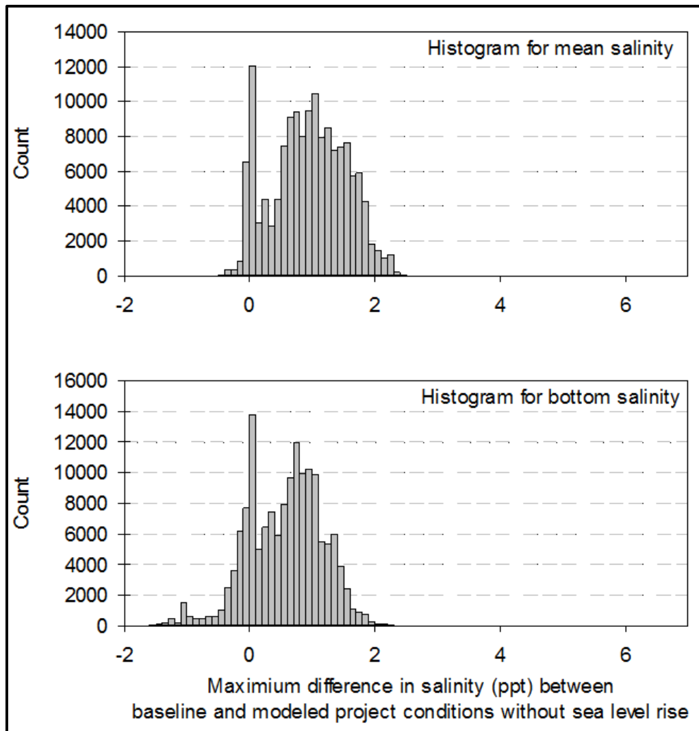
Figure 6-3. Maximum difference in model output between baseline and project conditions without SLR for mean and bottom salinity environmental parameters. Output values are based on intersect procedure between model grid and sample stations.
