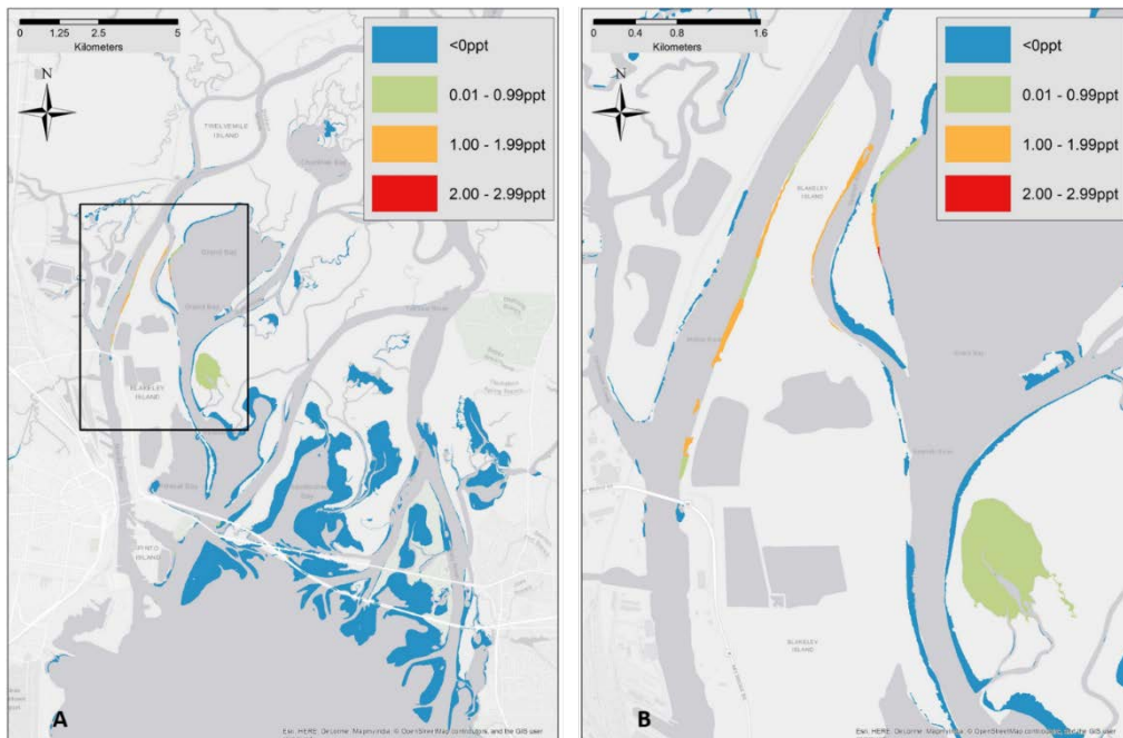
Figure 4-15. Change in salinity (ppt) above relative species-specific thresholds values from current baseline conditions to projected 0.5 m SLR conditions with no project implementation (i.e., SLR baseline – current baseline) within estuarine transition zone (A), and detailed within region of higher predicted salinity change (B, region outlined in black in A). SLR projections predict higher salinity increase than salinity increase due to project implementation alone.
