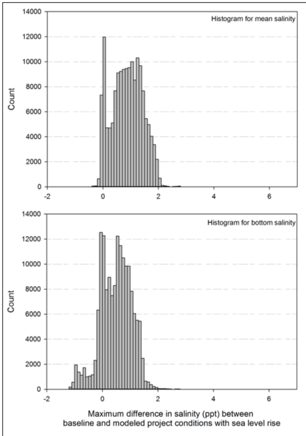
Figure 6-6. Maximum difference in model output between baseline and project conditions with SLR for mean and bottom salinity environmental parameters. Output values are based on intersect procedure between model grid and sample stations.
