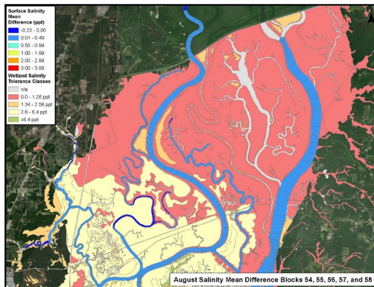
Figure 3-43. Estimated increase in salinity during the summer period (August data shown for example) within the upper (freshwater) portion of the study area. Note that estimated salinity increases are limited to 0.0, or <0.5 ppt. In areas where salinity increases may occur, wetland communities are adapted to predicted conditions. Map units designated n/a include upland habitats, highly disturbed and developed areas (e.g., historic fill, roads), and open water areas not addressed in the model domain.
