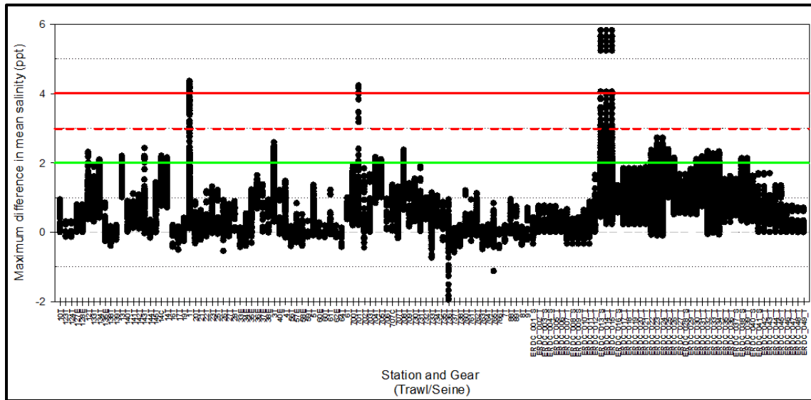
Figure 6-4. Model output for mean salinity (water column) with maximum difference in salinity (ppt) between baseline and modeled project conditions for all months at each designated AL Marine Resources and ERDC sample stations. Sampling station locations for codes in the x-axis are available on request. For each station, the vertical row of dots represents all of the intersected cells from the model grid across all months. The stations are arranged alphabetically by station number and there is no geographic perspective (i.e., upper, middle or lower Bay) portrayed by the order of the stations. Salinity differences with- and without-project are portrayed with reference lines at 2 (horizontal green line), 3 (horizontal dashed red line) and 4 ppt (solid horizontal red line).
