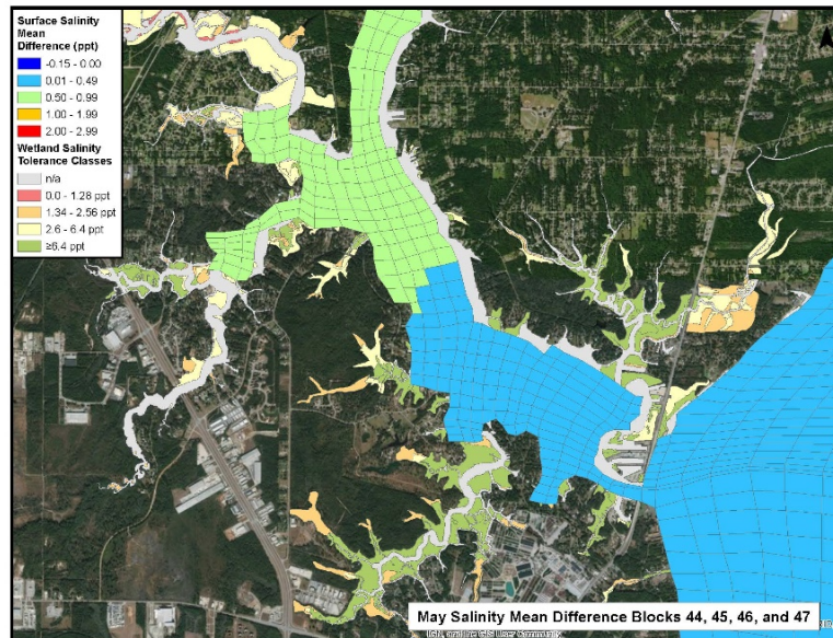
Figure 3-50. Estimated increase in salinity during the spring period (May data shown for example) within the lower (estuarine) portion of the study area. Note that in areas containing wetlands estimated salinity increases are limited to <0.5 or <1.0 ppt. In areas where increases may occur, wetland communities are adapted to predicted conditions. Map units designated n/a include upland habitats, highly disturbed and developed areas (e.g., historic fill, roads), and open water areas not addressed in the model domain.
