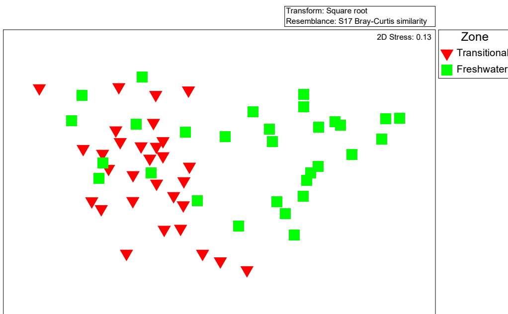
Figure 6-20. Non-metric multidimensional scaling plot of samples collected during fall sampling (October 2016) in the transitional (red symbols) and freshwater (green symbols) zones.
