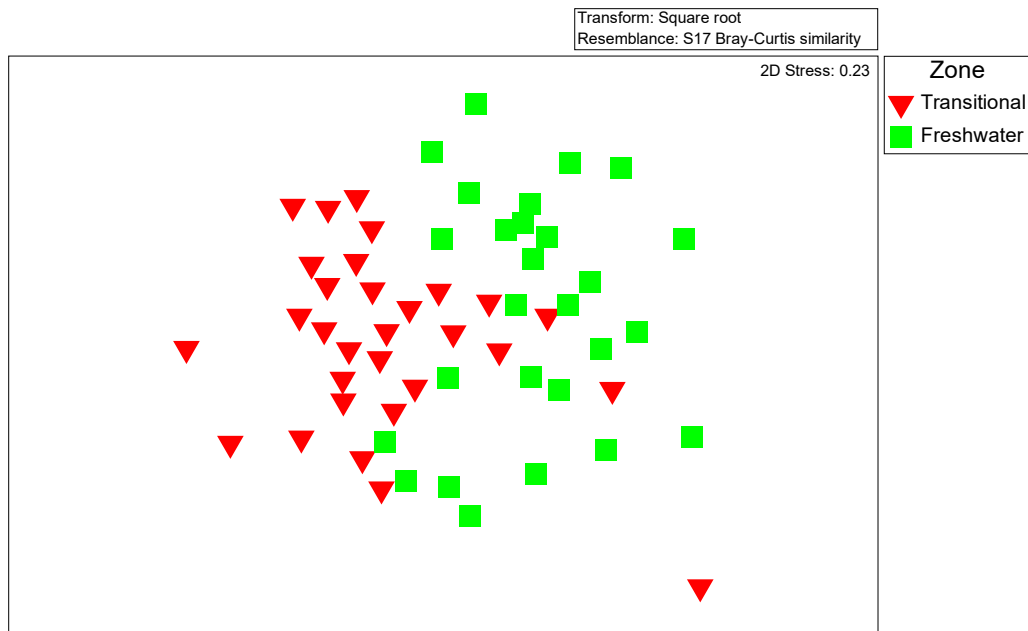
Figure 6-26. Non-metric multidimensional scaling plot of samples collected during spring sampling (May 2017) in the transitional (red symbols) and freshwater (green symbols) zones.
