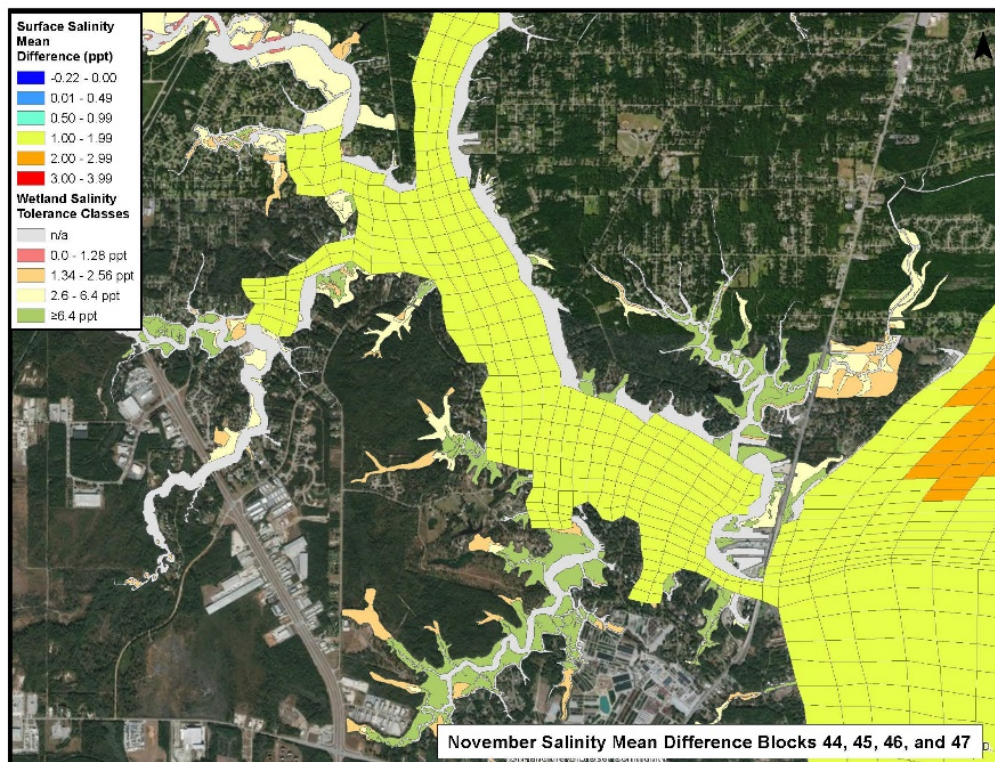
Figure 3-52. Estimated increase in salinity during the fall period (November data shown for example) within the lower (estuarine) portion of the study area. Note that in areas containing wetlands estimated salinity increases are limited to <1.0 ppt. In areas where increase occur, wetland communities are adapted to predicted conditions. Higher increases in salinity (e.g., <3.0 ppt) may occur adjacent to the navigation channel, but no wetlands are located in those areas (center right). Map units designated n/a include upland habitats, highly disturbed and developed areas (e.g., historic fill, roads), and open water areas not addressed in the model domain.
