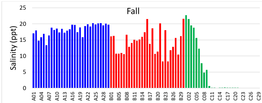
Figure 6-19. Non-metric multidimensional scaling plot of samples collected during fall sampling (October 2016) in the estuarine (blue symbols), transitional (red symbols), and freshwater (green symbols) zones. (below) Salinities at each station at the time of fall sampling.
