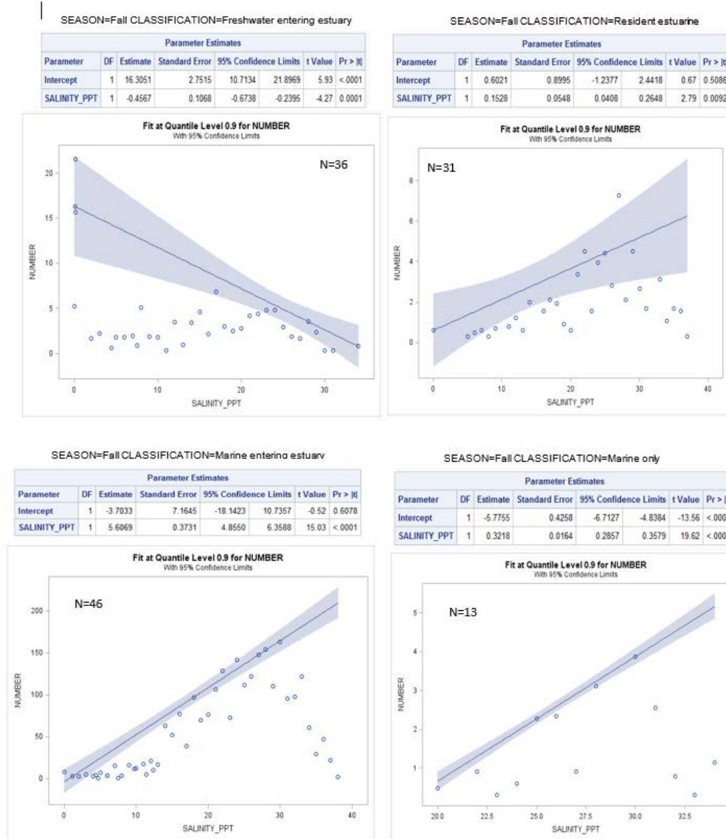
Figure 6-11. Quantile regression between numbers of fish classified according to salinity tolerance and salinity in ppt. The line indicates that the 90% quantile and the shaded portion is the 95% confidence interval around the regression line. Parameter estimates are provided along with the probability of significance. Figures are shown by season.
